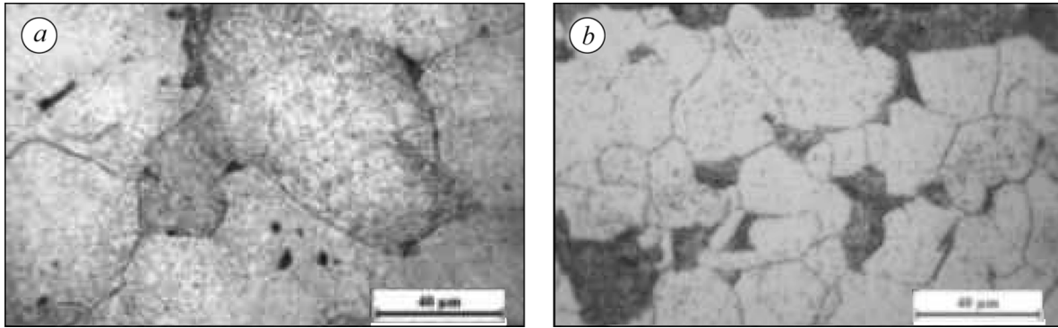
Fig. 8. Microstructures of the degraded PM (a) and new PM (b).
