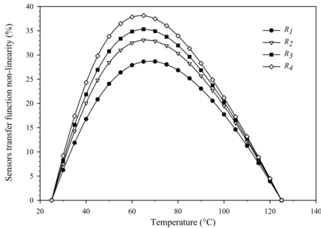
Fig. 13 Sensor transfer function non-linearity vs. temperature.
