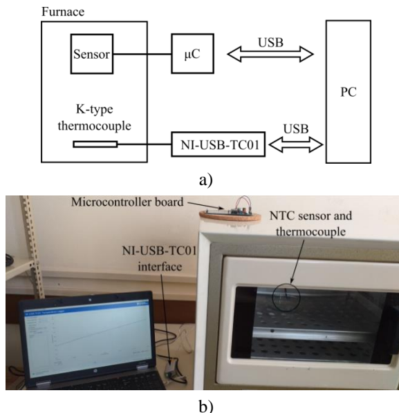
Fig. 12 Experimental setup: a) Block diagram, b) Photograph.
